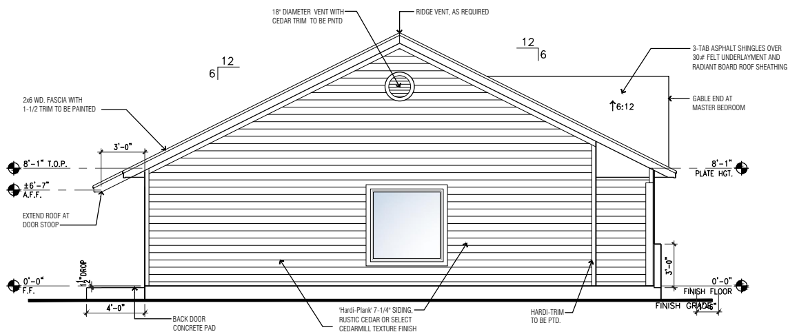
Side Elevations
