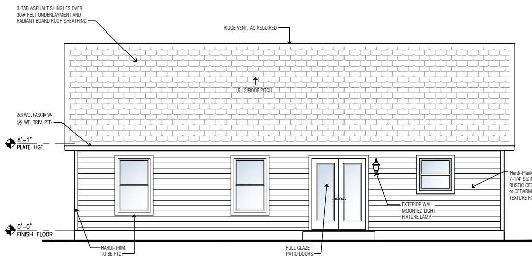
Rear Elevation
