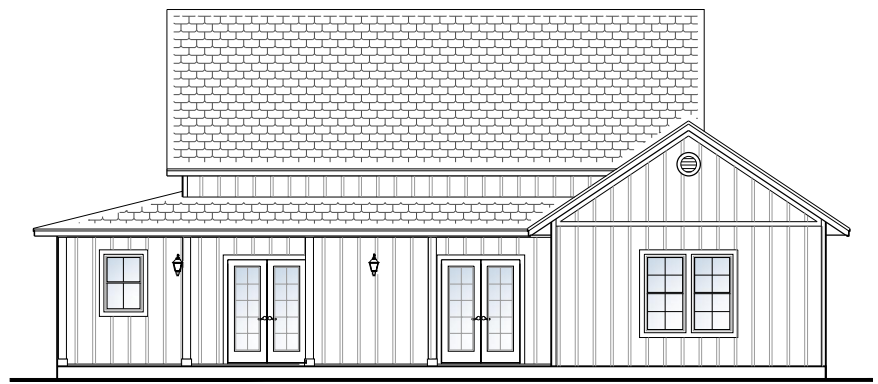
Rear Elevation
