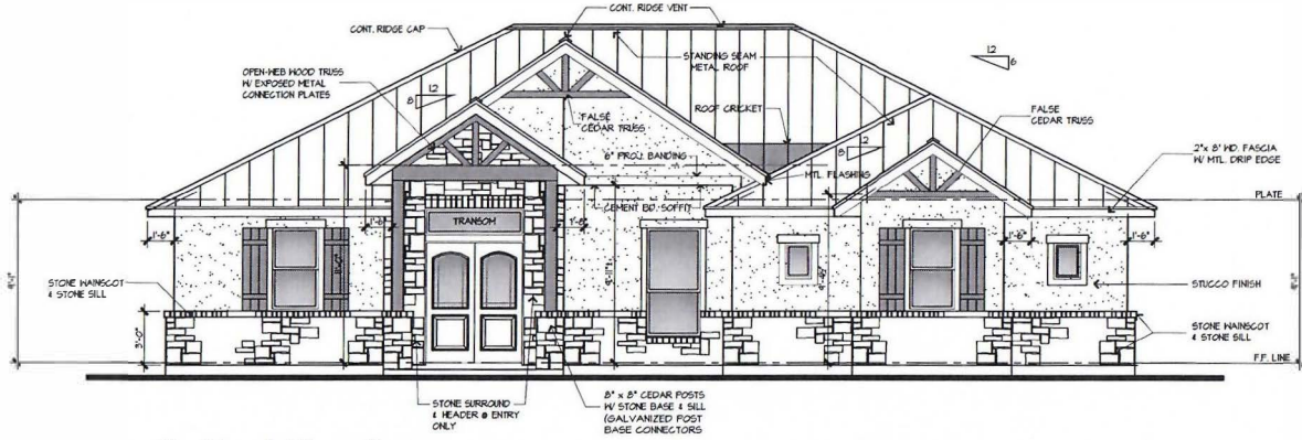
2. Front Elevation
